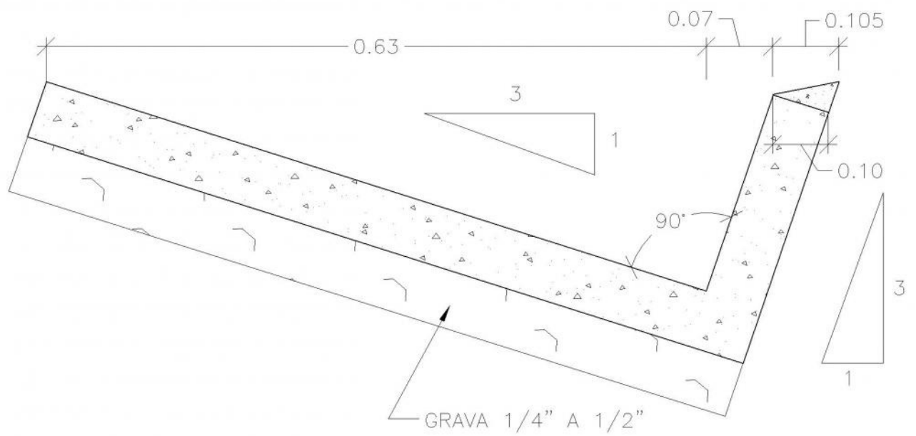
CUNETA SECCION TRIANGULAR
