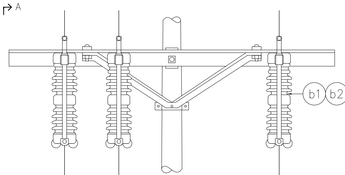
VISTA FRONTAL
