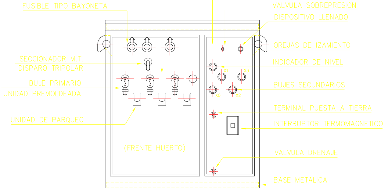
VISTA FRONTAL
